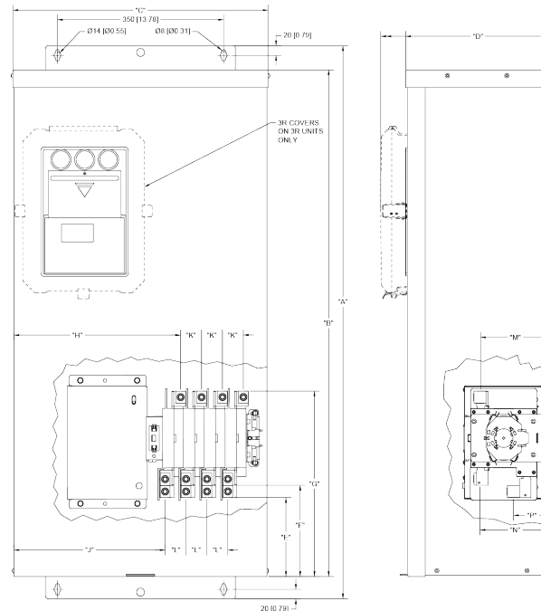
Contactor Type, Open and Delayed Transition, 100 – 400 A
